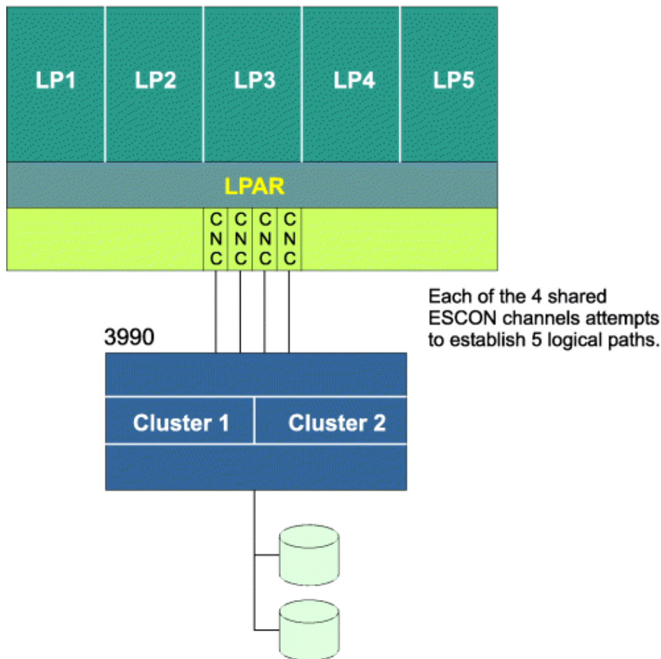
Figure 4. A shared ESCON configuration that can benefit from better logical path management
