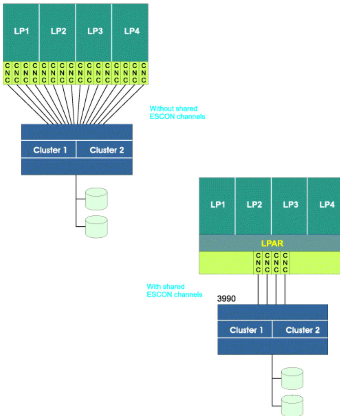
Figure 10. Consolidating ESCON channels and ESCON control unit ports
