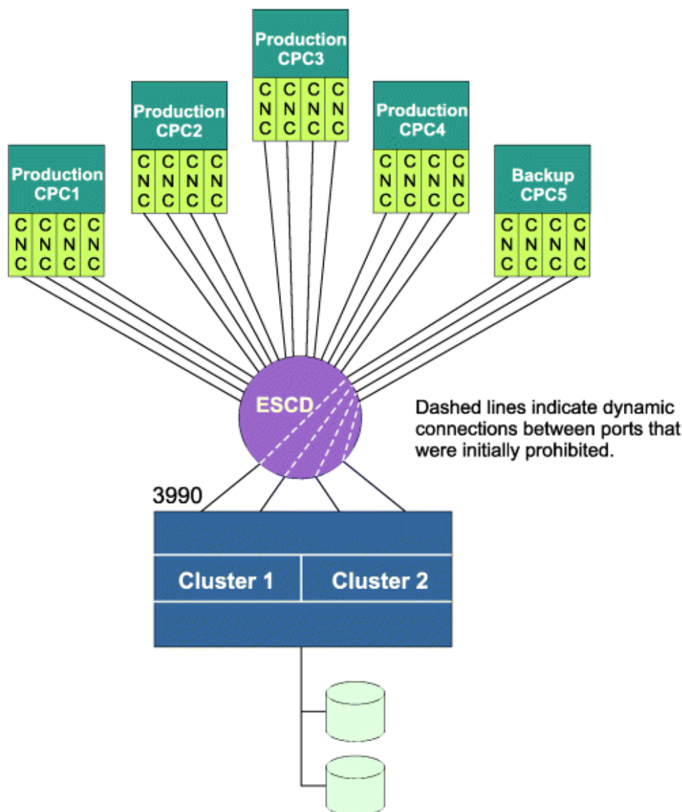
Figure 9. Using the ESCD to manage logical paths by prohibiting dynamic connections
