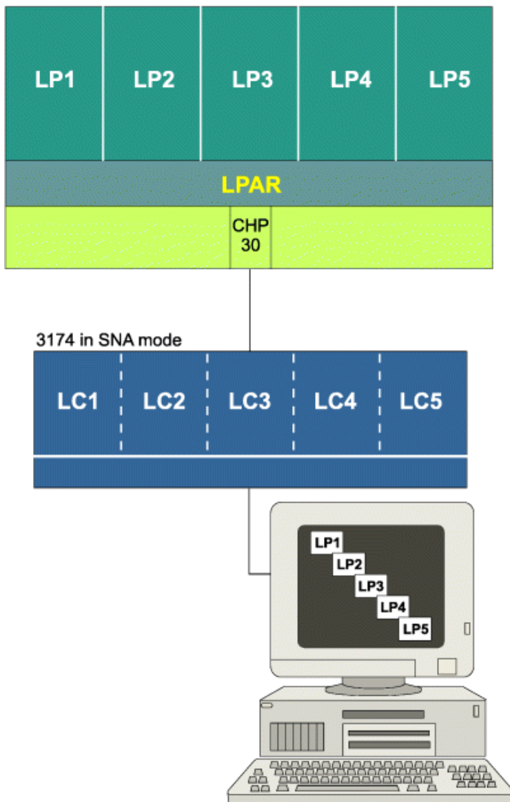
Figure 8. Defining devices to a subset of logical partitions
