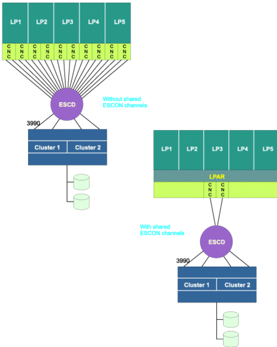
Figure 11. Consolidating ESCON channels and ESCD ports
