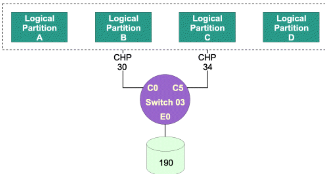
Figure 14. Shared devices using shared ESCON channels
